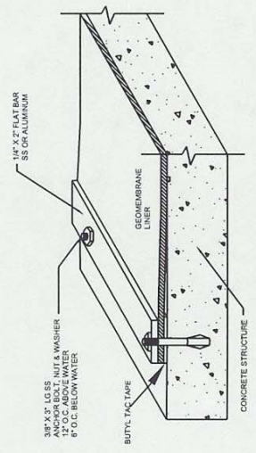
HORIZONTAL CONCRETE ANCHOR DETAIL TYP - NTS - DWG 0408
