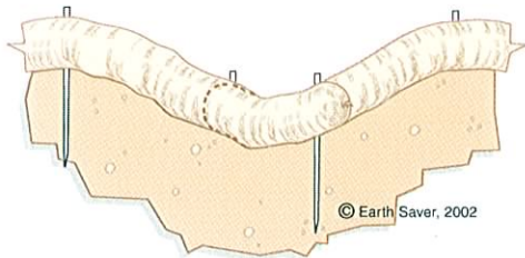
Typical Check Dam Application
